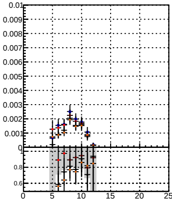
kFit_BDT_
