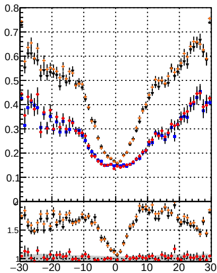
Fake rate vs d BDM Displaced SUSY CKFit BDM Displaced SUSY CKFit_BDT
