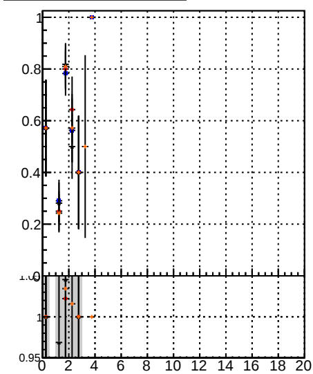
Fake rate vs. \chi^2 for various models and methods. The legend indicates: DOM Displaced SUSY CKE, DOM Displaced SUSY CKE Fit, DOM Displaced SUSY CKE BDT, and DOM Displaced SUSY CKE BDT.
