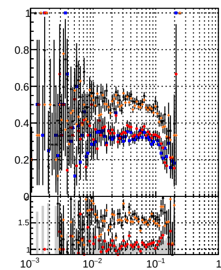
Fake rate vs DOM Displaced SUSY CKE CKEfit DOM Displaced SUSY CKE BDT DOM Displaced SUSY CKEfit BDT
