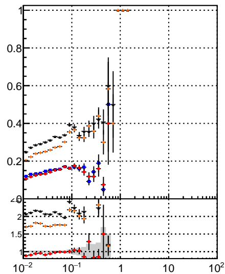
—•— DQM Displaced SUSY CKFit —•— DQM Displaced SUSY CKFit_BDT —•— DQM Displaced SUSY mKFit_BDT
