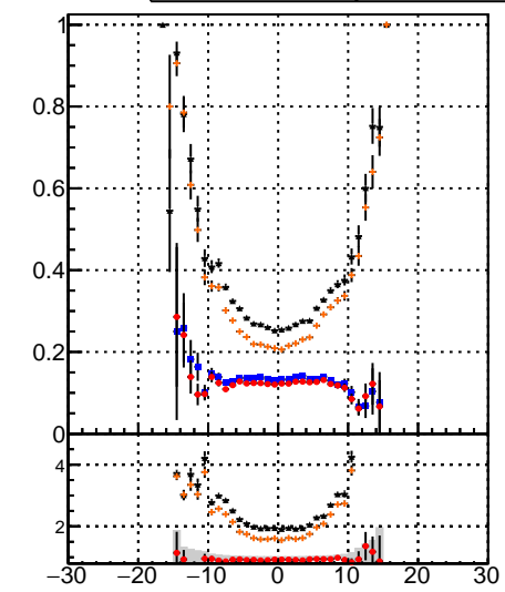
—•— DQM Displaced SUSY CKFit —•— DQM Displaced SUSY CKFit_BDT —•— DQM Displaced SUSY mKFit_BDT
