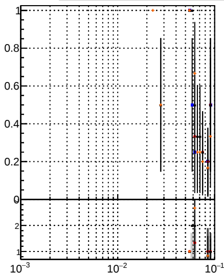
Fake rate vs DQM Displaced SUSY CKEfit DQM Displaced SUSY CKEfit BDT DQM Displaced SUSY mkFit BDT
