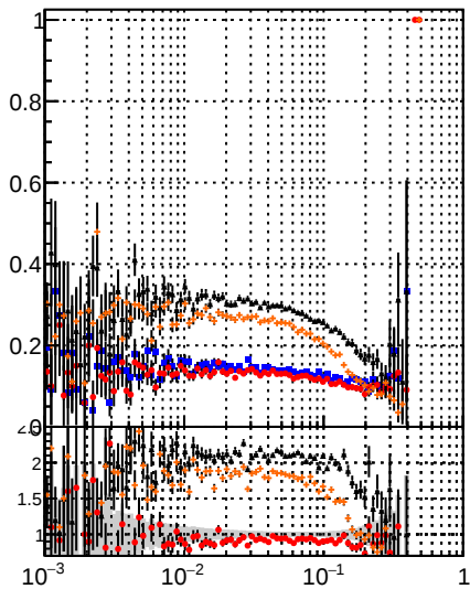
Fake rate vs DQM Displaced SUSY CKEfit DQM Displaced SUSY CKEfit BDT DQM Displaced SUSY mkFit BDT
