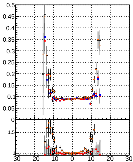
Fake rate vs d —●— BGM Displaced SUSY CKFit —●— BGM Displaced SUSY CKFit BDT —●— BGM Displaced SUSY CKFit BDT
