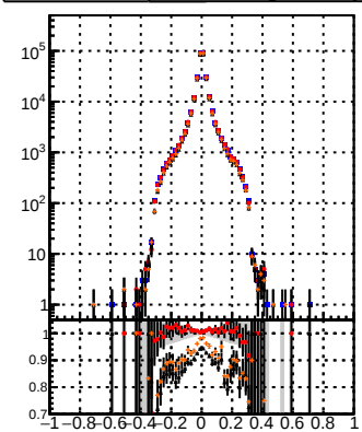
—●— DOM Displaced SUSY CKE —●— DOM Displaced SUSY CKE it —●— DOM Displaced SUSY mkt it BDT —●— DOM Displaced SUSY mkt it BDT
