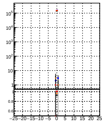
—●— DOM Displaced SUSY CKE —●— DOM Displaced SUSY CKE it —●— DOM Displaced SUSY mkt it BDT —●— DOM Displaced SUSY mkt it BDT
