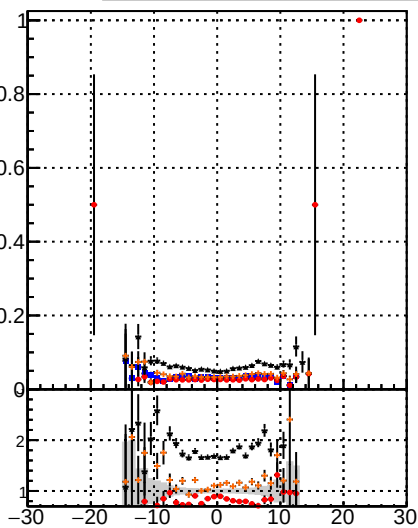
DOM Displaced SUSY CKE DOM Displaced SUSY CKEfit DOM Displaced SUSY BDT DOM Displaced SUSY mkFit BDT
