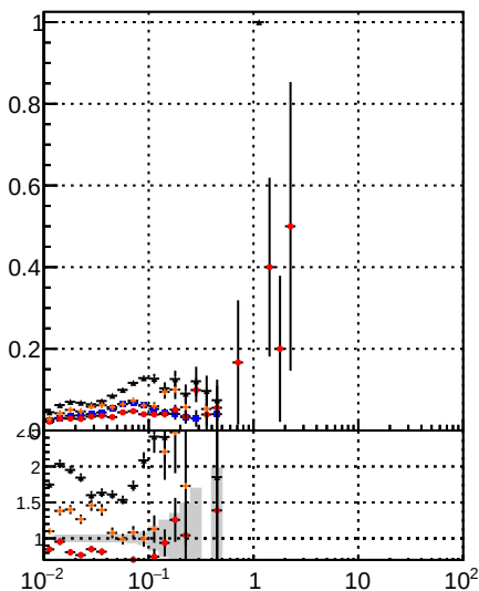
DOM Displaced SUSY CKE DOM Displaced SUSY CKEfit DOM Displaced SUSY BDT DOM Displaced SUSY mkFit BDT
