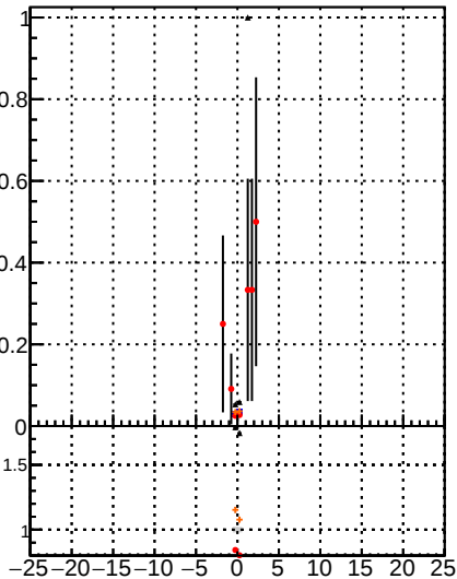
Fake rate vs d —●— BSM Displaced SUSY CKE —●— BSM Displaced SUSY CKE fit —●— BSM Displaced SUSY CKE fit BDT
