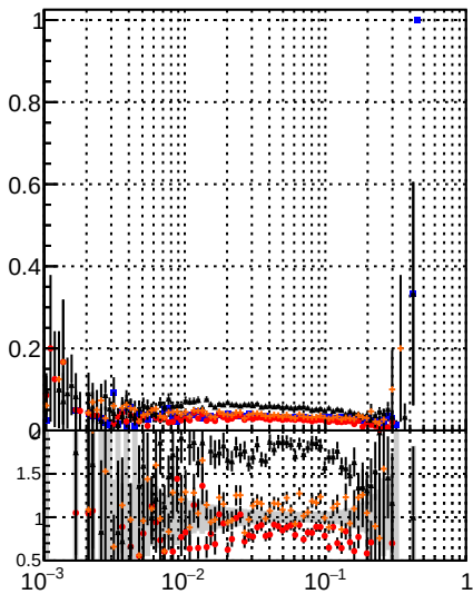
Fake rate vs DOM Displaced SUSY CKE DOM Displaced SUSY CKE fit DOM Displaced SUSY mkFit BDT
