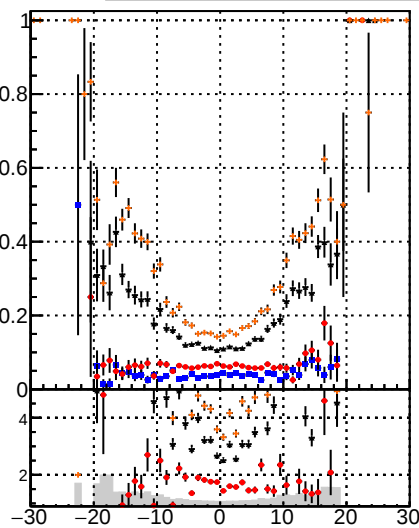
Fake rate vs \nu DOM Displaced SUSY CKE DOM Displaced SUSY CKEfit DOM Displaced SUSY BDT DOM Displaced SUSY mkFit BDT
