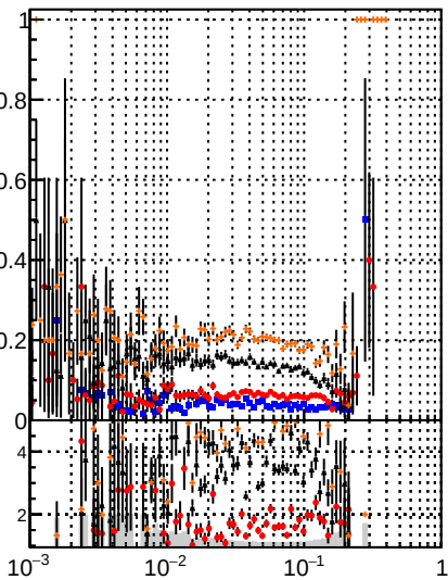
Fake rate vs DOM Displaced SUSY CKE DOM Displaced SUSY CKEfit DOM Displaced SUSY CKEfit_BDT DOM Displaced SUSY mkFit_BDT
