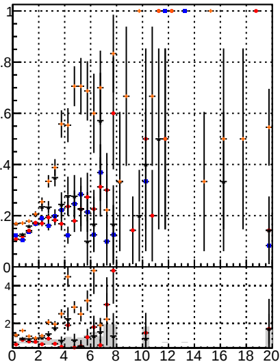
Fake rate vs. — BDM Displaced SUSY CKFit CKFit_BDT — BDM Displaced SUSY CKFit CKFit_BDT
