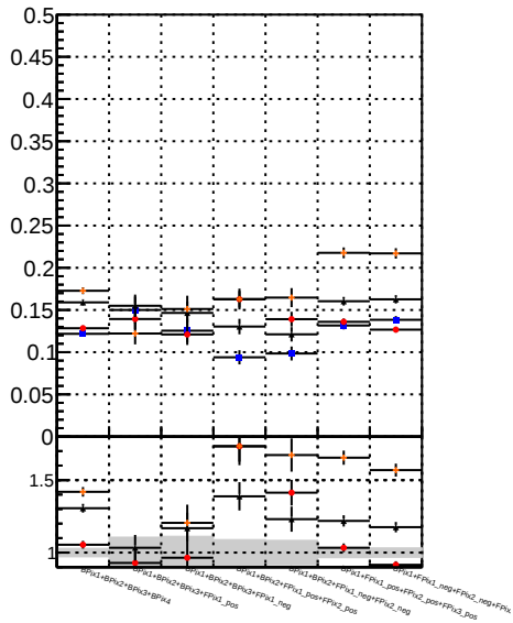
Fake rate vs. — BDM Displaced SUSY CKFit CKFit_BDT — BDM Displaced SUSY CKFit CKFit_BDT
