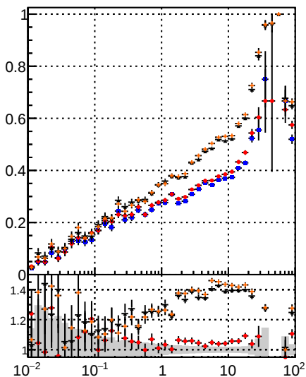
Fake rate vs \nu DOM Displaced SUSY CKE DOM Displaced SUSY CKE fit DOM Displaced SUSY mkt fit BDT
