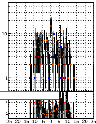
N of associated (recoToSim) loop tracks vs dxy
