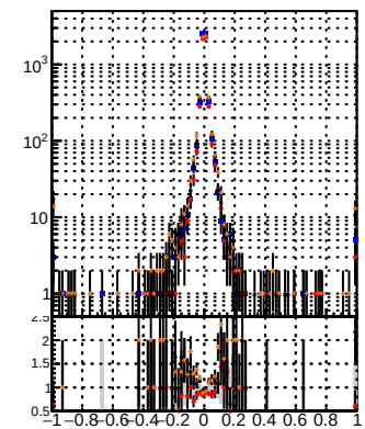
— DOM Displaced SUSY CKE — Displaced SUSY CKE mkt BDT — DOM Displaced SUSY CKE mkt BDT
