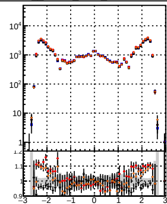
N of reco track vs \eta BQM Displaced SUSY GKF MKFit BDT BQM Displaced SUSY GKF MKFit BDT
