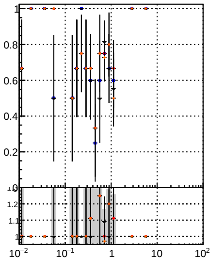
Fake rate vs \sqrt{s} Legend: DQM Displaced SUSY (blue circles) CKE (orange circles) BDT (red circles)
