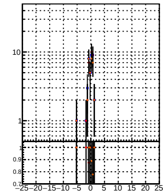
N of reco track vs dxy(PV) vs dxy(PV) DQM Displaced SUSY CKE mkFit BDT DQM Displaced SUSY CKE mkFit BDT
