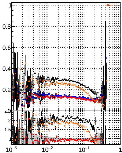
—•— DOM Displaced SUSY CKEfit —•— DOM Displaced SUSY CKEfit_BDT —•— DOM Displaced SUSY mkFit_BDT
