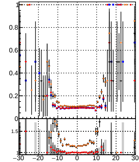
DOM Displaced SUSY CKE DOM Displaced SUSY CKEfit DOM Displaced SUSY mkFit BDT
