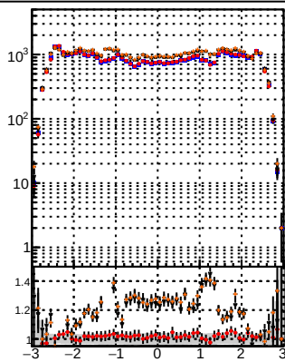
N of reco track vs \eta p_T [GeV]
