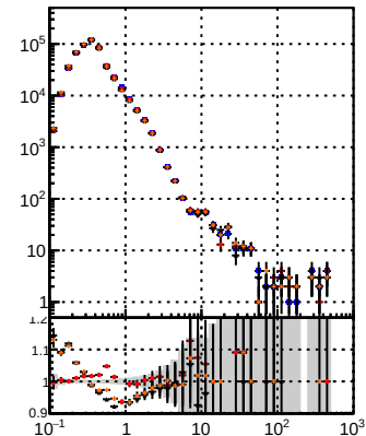
N of reco track vs \eta p_T [GeV]
