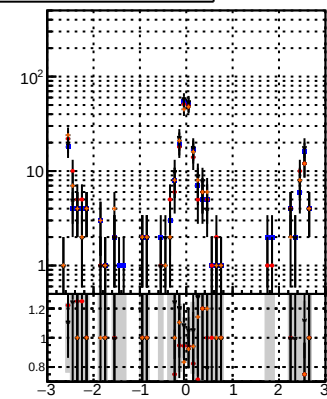
N of reco track vs \eta p_T [GeV]
