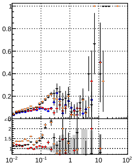
Fake rate vs \nu DOM Displaced SUSY CKE DOM Displaced SUSY CKEfit DOM Displaced SUSY BDT DOM Displaced SUSY mkFit BDT
