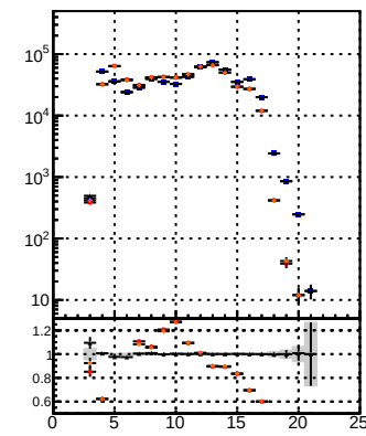
DOM Displaced SUSY CKE DOM Displaced SUSY mke-it DOM Displaced SUSY mke-it BDT
