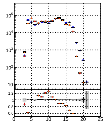
DOM Displaced SUSY CKE DOM Displaced SUSY mke-it DOM Displaced SUSY mke-it BDT
