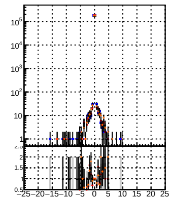
—•— DOM Displaced SUSY CKE —•— DOM Displaced SUSY mkt-fit BDT —•— DOM Displaced SUSY CKEit BDT
