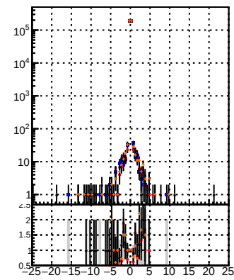
—•— DOM Displaced SUSY CKE —•— DOM Displaced SUSY mkt-fit BDT —•— DOM Displaced SUSY CKEit BDT
