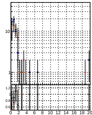
N of associated (recoToSim) lepton tracks vs normalized \chi^2
