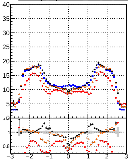
mean hit Legend: Blue line: DQM_DisplacedSUSY CKF Red line: DQM_DisplacedSUSY mkFit Black line: DQM_DisplacedSUSY CKF_BDT Orange line: DQM_DisplacedSUSY mkFit_BDT
