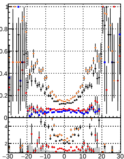
Fake rate vs d DGM Displaced SUSY CKFit DGM Displaced SUSY CKFit+BDT
