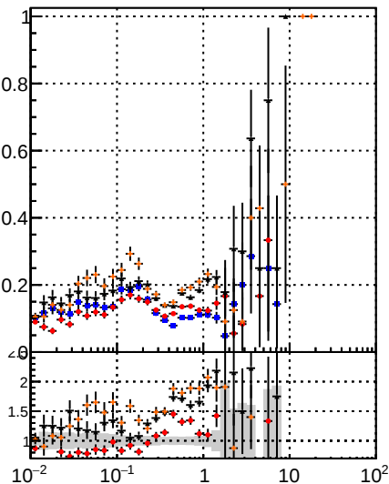
DOM Displaced SUSY CKE DOM Displaced SUSY CKE fit DOM Displaced SUSY CKE fit BDT DOM Displaced SUSY mkFit BDT
