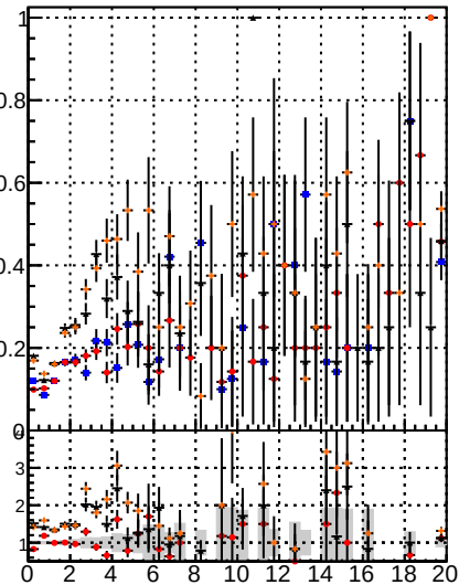
Fake rate vs. BSM Displaced SUSY CKFit_BDT BSM Displaced SUSY CKFit BSM Displaced SUSY BSM Displaced SUSY CKFit_BDT
