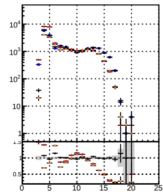
—●— DOM Displaced SUSY CKE —●— DOM Displaced SUSY mkt-fit —●— DOM Displaced SUSY mkt-fit BDT
