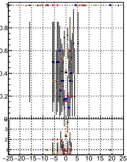
Fake rate vs dxy —●— BGM Displaced SUSY CKF —●— BGM Displaced SUSY CKFit —●— BGM Displaced SUSY CKFit_BDT
