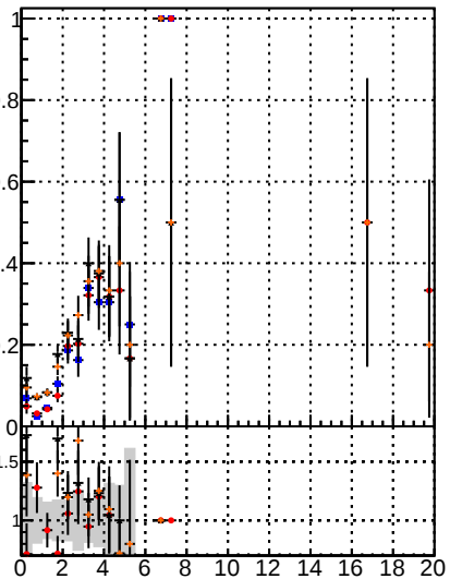
Fake rate vs. DOM Displaced SUSY GKE CKE BDT
