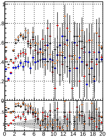
Fake rate vs. BSM Displaced SUSY CKFit BSM Displaced SUSY CKFit_BDT BSM Displaced SUSY CKFit_BDT
