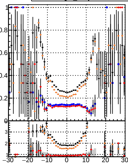
— DOM Displaced SUSY CKE — DOM Displaced SUSY CKE fit — DOM Displaced SUSY CKE fit BDT — DOM Displaced SUSY CKE fit BDT
