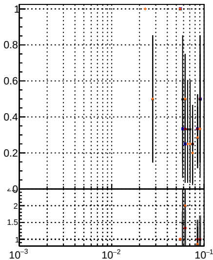
—•— DQM Displaced SUSY CKE —•— DQM Displaced SUSY CKEfit —•— DQM Displaced SUSY CKEfit BDT —•— DQM Displaced SUSY mkFit BDT
