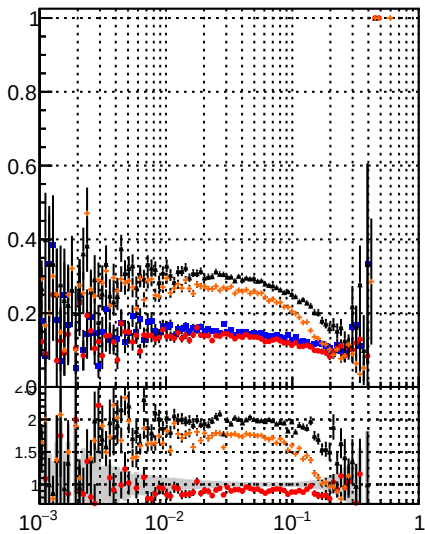
—•— DQM Displaced SUSY CKE —•— DQM Displaced SUSY CKEfit —•— DQM Displaced SUSY CKEfit BDT —•— DQM Displaced SUSY mkFit BDT
