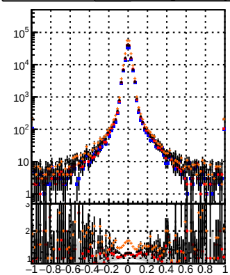
—●— DOM Displaced SUSY CKE —●— DOM Displaced SUSY CKE+it —●— DOM Displaced SUSY CKE+it+BDT —●— DOM Displaced SUSY CKE+it+BDT
