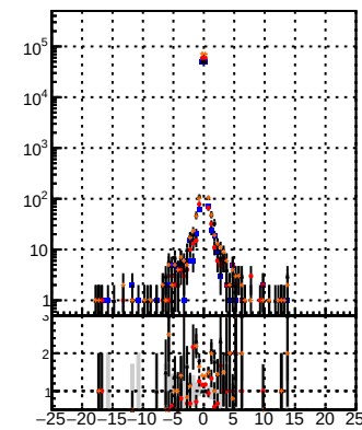
—●— DOM Displaced SUSY CKE —●— DOM Displaced SUSY CKE+it —●— DOM Displaced SUSY CKE+it+BDT —●— DOM Displaced SUSY CKE+it+BDT
