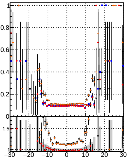
DOM Displaced SUSY CKFit DOM Displaced SUSY CKFit DOM Displaced SUSY CKFit BDT DOM Displaced SUSY CKFit BDT
