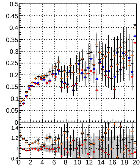
Fake rate vs. BGM Displaced SUSY CKE Fit BGM Displaced SUSY CKE Fit BGM Displaced SUSY CKE Fit
