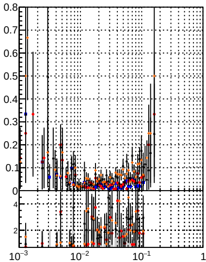
DOM Displaced SUSY CKEfit Displaced SUSY CKEfit BDT Fake rate vs dr
