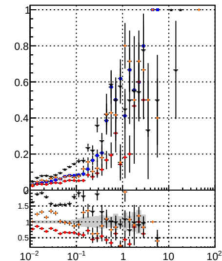
—•— DOM Displaced SUSY CKE —•— DOM Displaced SUSY CKE fit —•— DOM Displaced SUSY CKE fit BDT
