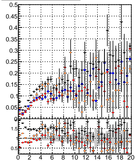
Fake rate vs. DCM Displaced SUSY CKFit CKFit_BDT DCM Displaced SUSY CKFit CKFit_BDT
