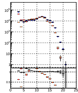
DOM Displaced SUSY CKE Displaced SUSY mkt Displaced SUSY mkt+BDT Displaced SUSY CKE+BDT
