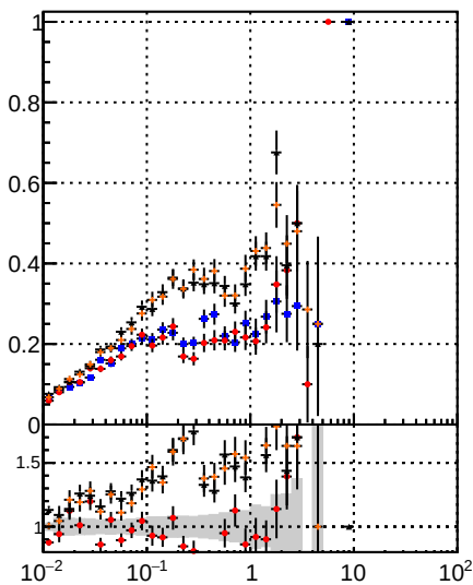
DOM Displaced SUSY CKE DOM Displaced SUSY CKE fit DOM Displaced SUSY CKE fit BDT Fake rate vs v
