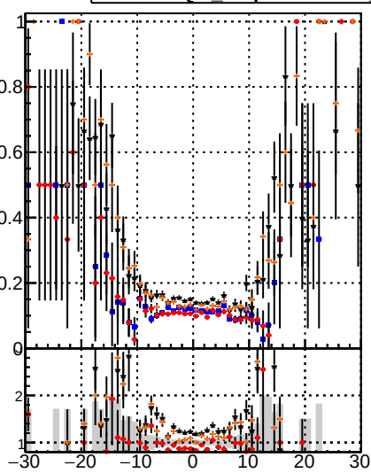
DOM Displaced SUSY CKE DOM Displaced SUSY CKE fit DOM Displaced SUSY CKE fit BDT Fake rate vs v
