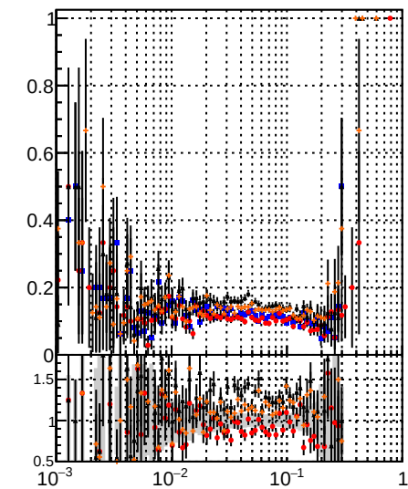
DOM Displaced SUSY CKE DOM Displaced SUSY CKE fit DOM Displaced SUSY CKE fit BDT DOM Displaced SUSY CKE fit BDT
