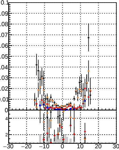
Duplicates Rate vs sim PV z
