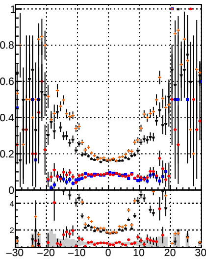
Fake rate vs v DOM Displaced SUSY CKE DOM Displaced SUSY CKE fit DOM Displaced SUSY BDT DOM Displaced SUSY mkFit BDT
