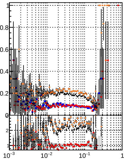
Fake rate vs DOM DisplacedSUSY CKE BDT DOM DisplacedSUSY CKE BDT DOM DisplacedSUSY CKE BDT
