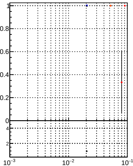
Fake rate vs DOM DisplacedSUSY CKE BDT DOM DisplacedSUSY CKE BDT DOM DisplacedSUSY CKE BDT
