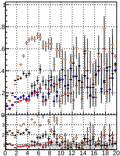
Fake rate vs. — BDM Displaced SUSY CKFit — BDM Displaced SUSY CKFit_BDT — BDM Displaced SUSY mFit_BDT
