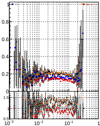
Fake rate vs DOM Displaced SUSY CKE CKEfit BDT DOM Displaced SUSY CKEfit BDT
